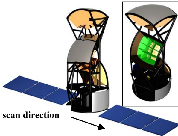
FIGURE 1. a) EXIST telescopes (3) on spacecraft, zenith pointed along orbital scan direction, b) cutaway view showing imaging CZT detector arrays and active collimator.
