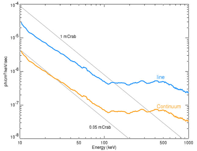
FIGURE 2. EXIST survey sensitivities. GRB sensitivities are \sim 50\text{mCrab} for an assumed 10sec duration burst.
