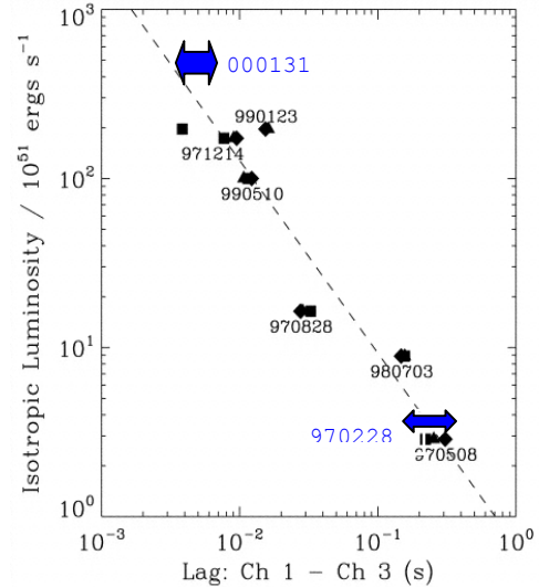
FIGURE 4. Luminosity-lag relation for GRBs (adapted from [7]). The observed correlation, L_{\text{pk}} \propto \Delta\tau^{-1.14} , may be understood as a kinematic effect from beaming [8].
