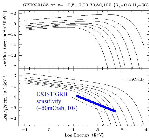
FIGURE 3. GRB sensitivity vs. z (adapted from [3]).
